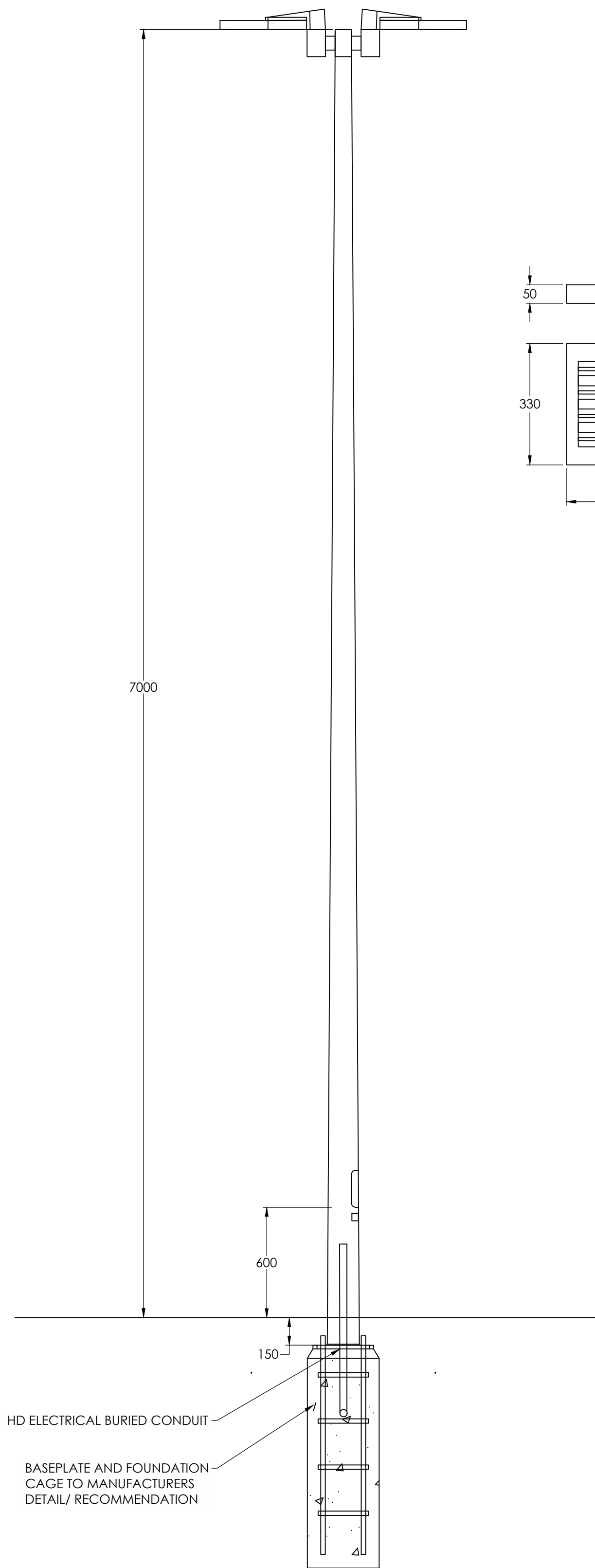
03 POLE SIDE ELEVATION - [A2, A3] 1:20@A1
