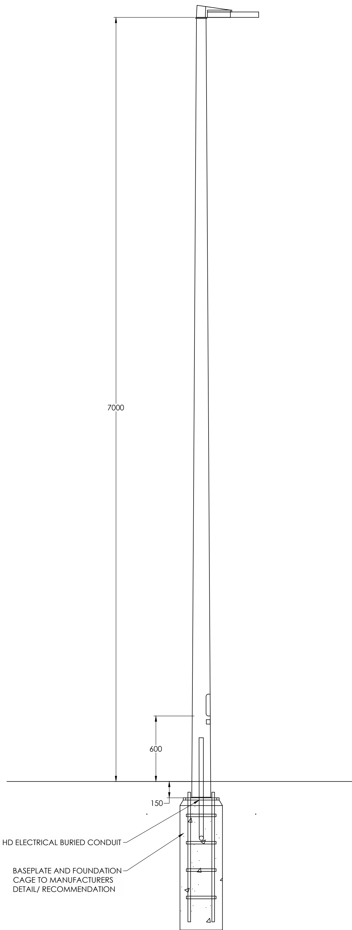
02 POLE SIDE ELEVATION - [A1, A4, B1] 1:20@A1
