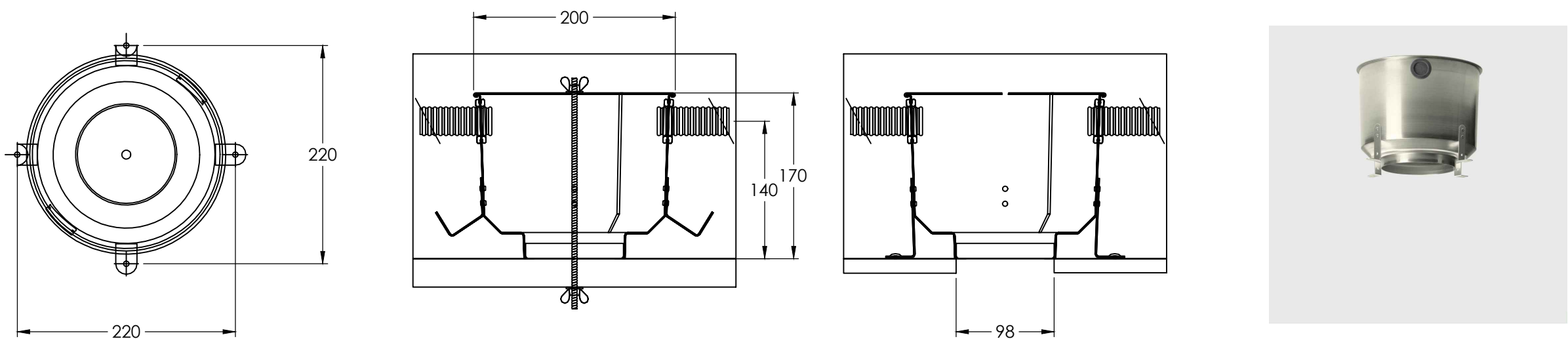
02 DL3 - CONCRETE HOUSING 1:5@A1
