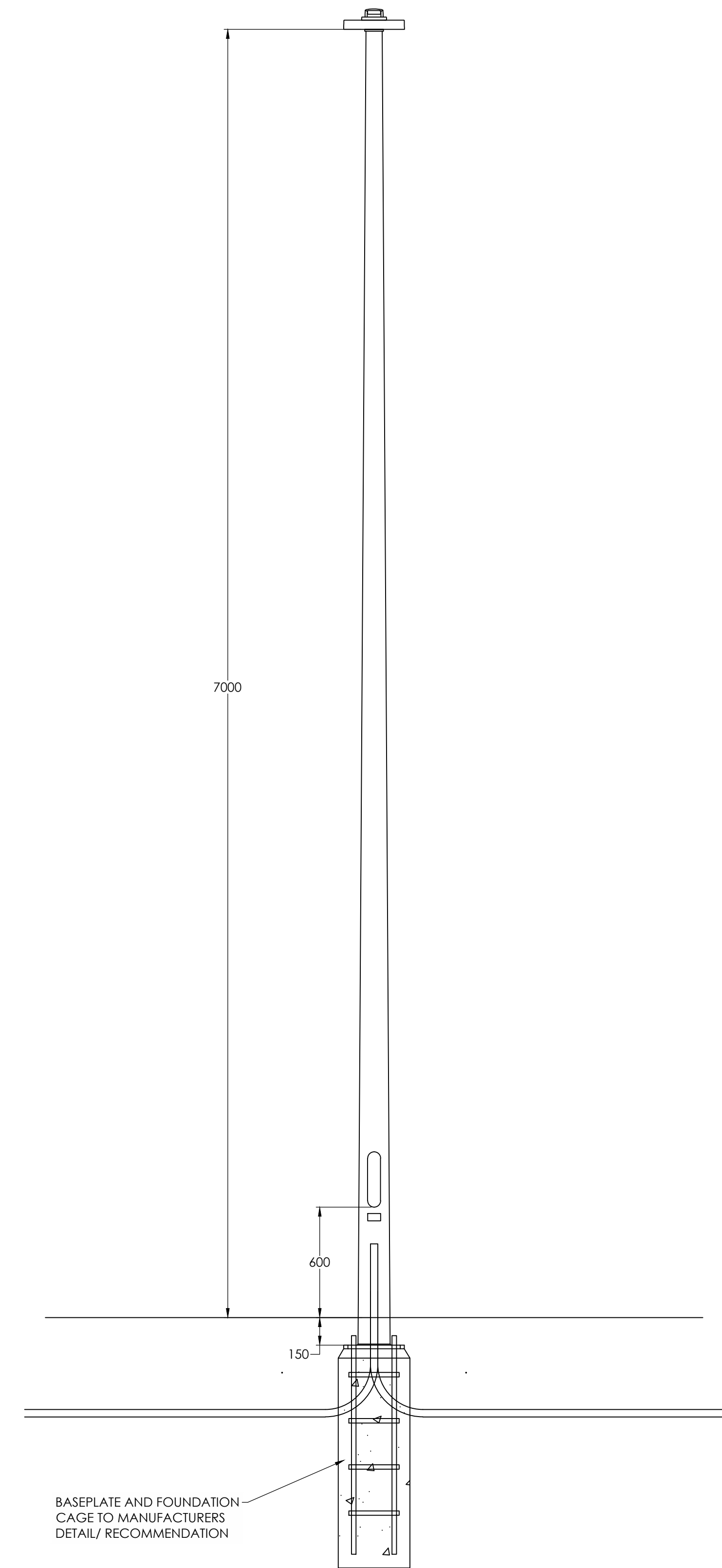
01 POLE FRONT ELEVATION - [A1, A4, B1] 1:20@A1
