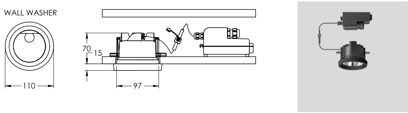
01 LUMINAIRE DETAILS - DOWNLIGHTS [DL3] 1:5@A1
